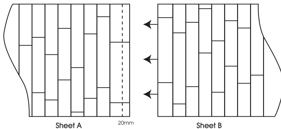
Diagram 2 - Overlap Sheet B over Sheet A by 20mm (to dotted line indicated) and cut in the joint. The end plank on one side is 20mm wider than the rest of the planks to enable this.
